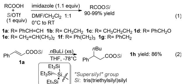
Scheme 1. Supersilyl ester synthesis and the 1,4-addition reaction.
